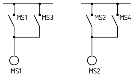
Sensor group 1
